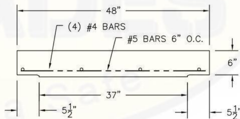
COVER DETAIL
