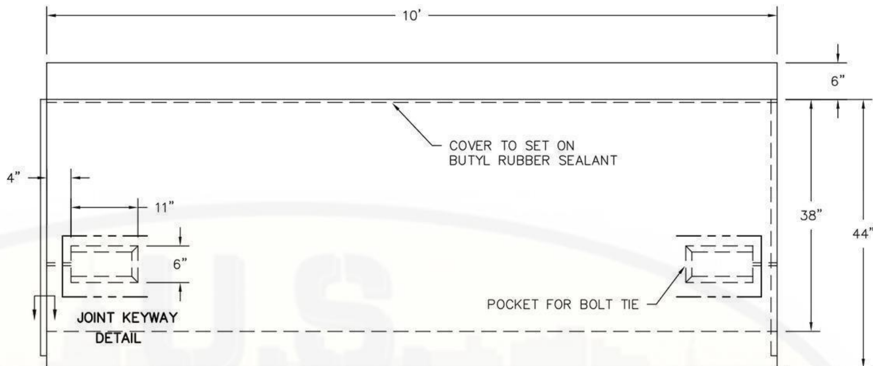
SIDE VIEW
