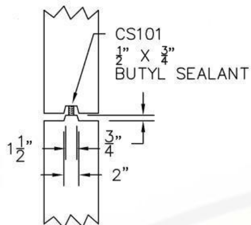
JOINT KEY WAY DETAIL
