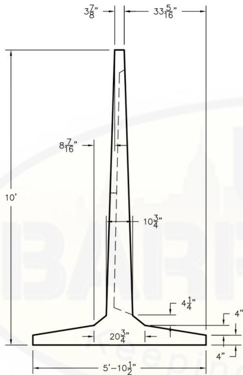
END ELEVATION VIEW
