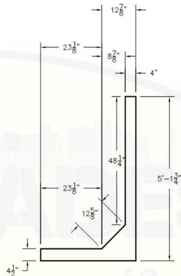
END VIEW
