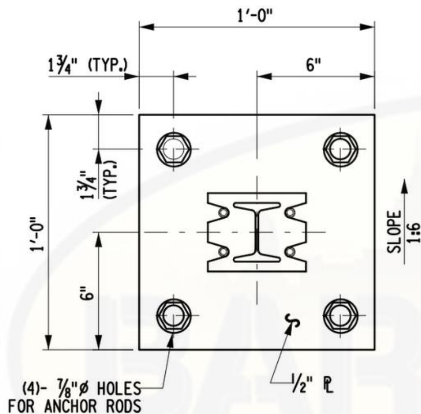
ANCHOR POST BASE DETAIL PLAN VIEW
