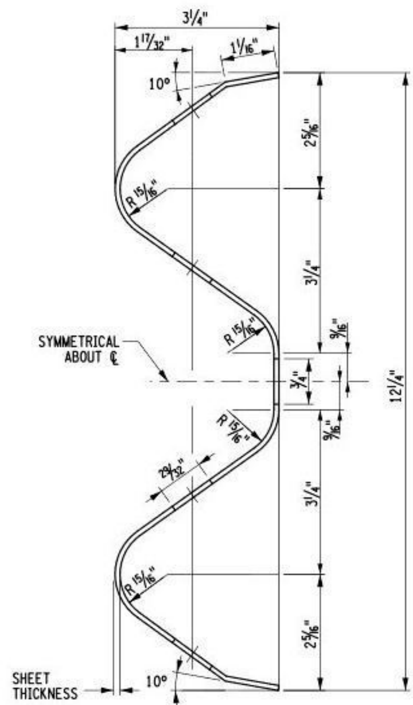
RAIL ELEMENT DETAIL
