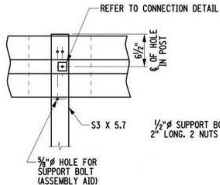
BEAM MOUNTING
