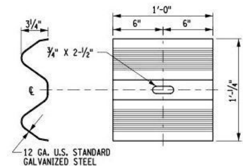
GUIDE RAIL POST BACKUP PLATE
