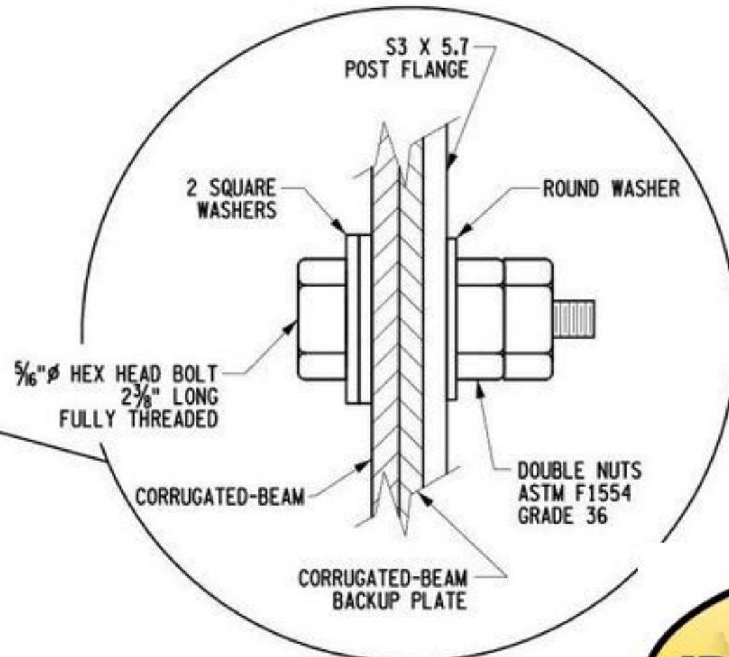
CONNECTION DETAIL
